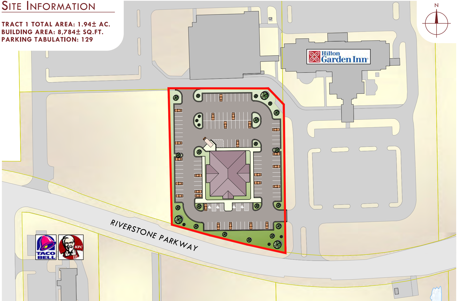
SITE CONCEPT PLAN • OPTION 1 • TRACT 1 RIVERSTONE PARKWAY • KANKAKEE, ILLINOIS
